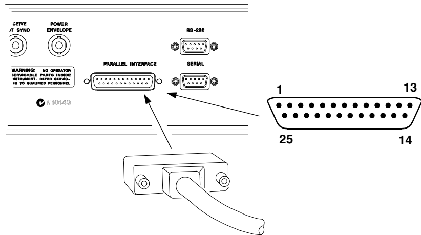
Parallel Interface - male connector configuration.
